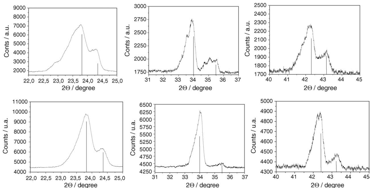
Fig. 3. Details of the BA peaks of Fig. 2; the upper three are for the MA sample, the lower ones are the corresponding angle peaks for the as-received sample.
