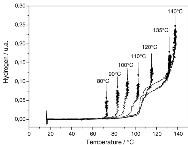
Fig. 9. The amount of hydrogen released from the 1 mol% doped sample as a function of the sample temperature. The nominal temperature is also reported.
