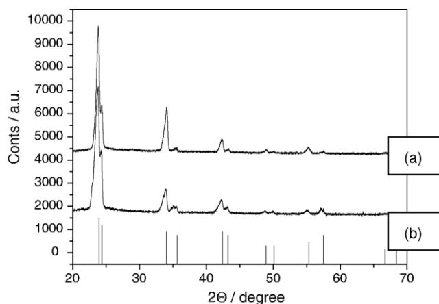
Fig. 2. XRD spectra of as-received (a) and MA (b) \text{NH}_3\text{BH}_3 sample.
