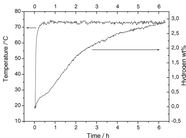
Fig. 7. Time evolution of hydrogen desorption for the 1% doped sample heated at 73 °C.
