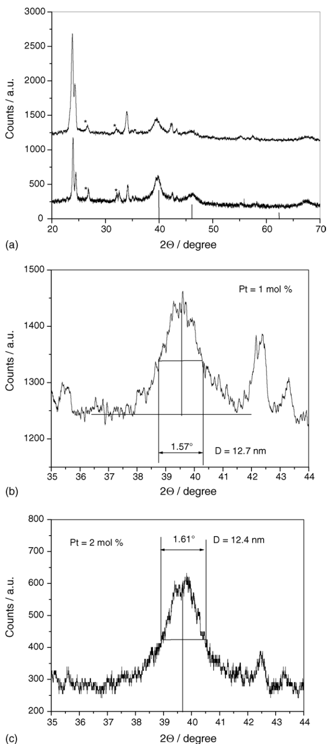
Fig. 4. (a) XRD spectra for the 1 and 2 mol% platinum MR samples; (b, c) zooms of the peaks in (a) related to [1 1 1]Pt.
