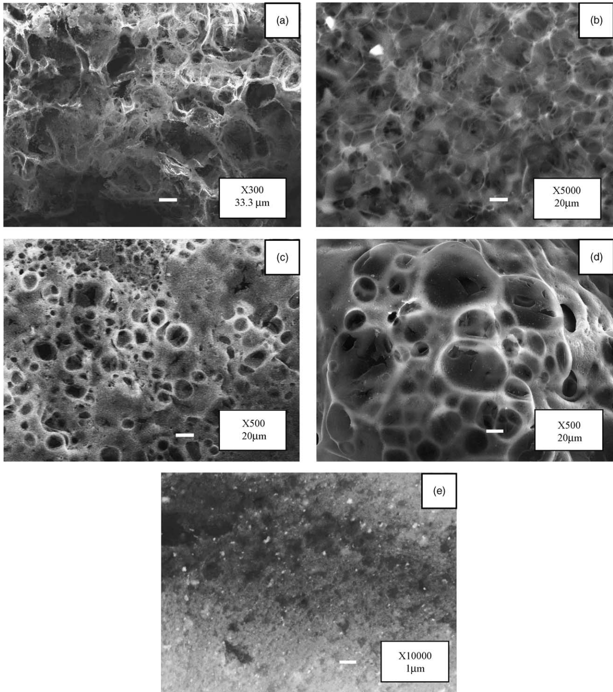
Fig. 5. SEM images of as-received BA (a), ball milled BA (b), with 1 mol% H 2 PtCl 6 (c, e), with 2 mol% H 2 PtCl 6 (d).
