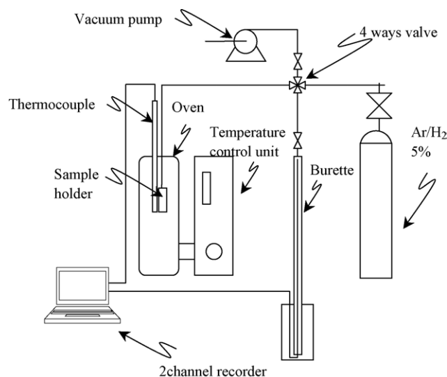
Fig. 1. The experimental apparatus for thermal decomposition measurements.
