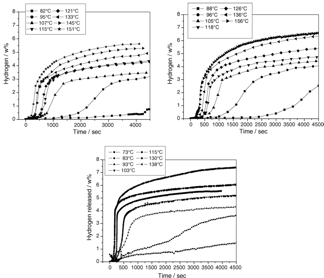
Fig. 6. Time evolution of the decomposition reaction of BA complex as-received (a), after MA (b) and MR with 1 mol% Pt (c).
