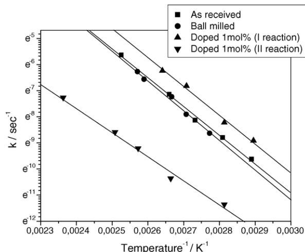
Fig. 8. Arrhenius plot of the kinetic constants.
